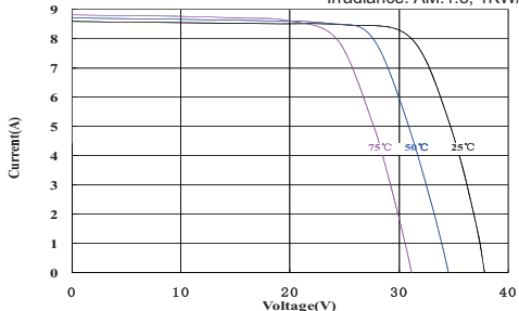
I-V Curves of CNPV-255MB at different cell temperature Irradiance: AM.1.5, 1KW/ m 2
